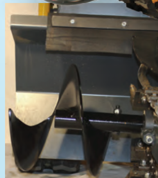
Soil evacuation with auger
